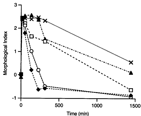
Figure 5. Change in morphological index. Erythrocytes were converted into echinocytes by addition of DLPC (35 \mu\text{M} ) at t = 0 , then at t = 15 min separate batches were treated with 35 \mu\text{M} of sulfonamide 1 (filled diamonds), amide 2 (open circles), ester 3 (open squares), chlorpromazine (filled triangles), and no addition (crosses) at pH 7.4 and T = 37 ^{\circ}\text{C} . Each point is the average of three independent runs, with an uncertainty of \pm 0.3 morphological index units.
